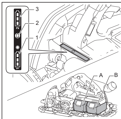
► 1. Battery indicator (battery A) 2. Check button 3. Battery indicator (battery B)
