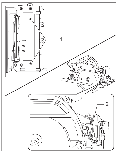
► 1. Adjusting screw for 0° angle 2. Adjusting screw for 45° angle
